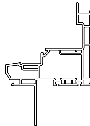
SECTION VIEW C-C ALTERNATE FIN ONLY FRAME
