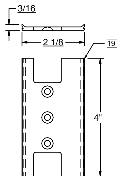
Panel Guide, Interlock - P-5517
