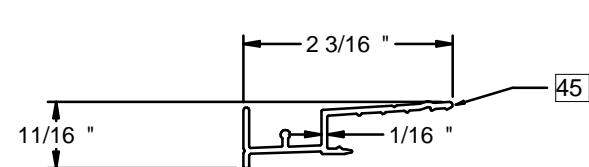
Screen, 1-Track Sill - 2134
