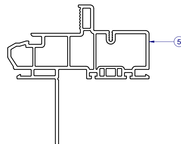
ALTERNATE FIN ONLY FRAME
