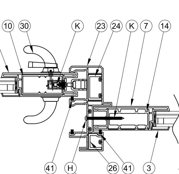
6 HORIZONTAL CROSS SECTION 3 MULLION (OFFSET BUTTSTILE)
