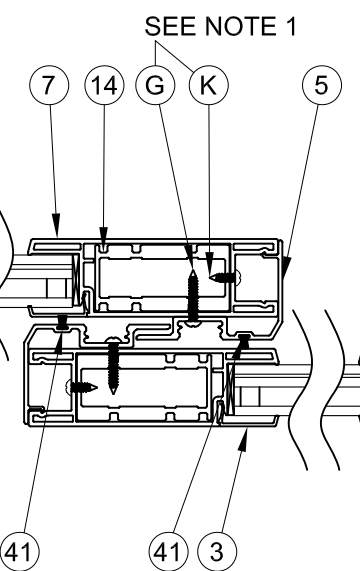
2 HORIZONTAL CROSS SECTION 3 INTERLOCK
