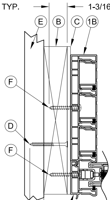
2 HORIZONTAL CROSS SECTION 3 INTERLOCK
