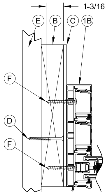
1 HORIZONTAL CROSS SECTION 3 2X BUCK CONSTRUCTION
