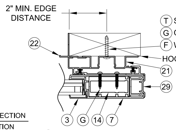
8 HORIZONTAL CROSS SECTION 3 HOOKSTRIP
