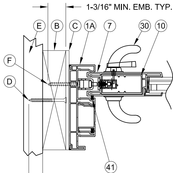
1 HORIZONTAL CROSS SECTION 3 2X BUCK CONSTRUCTION
