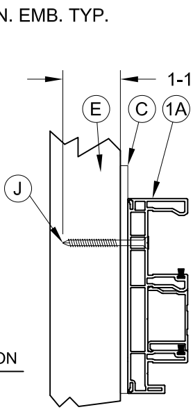
10 HORIZONTAL CROSS SECTION 3 MASONRY CONSTRUCTION SEE NOTE 5
