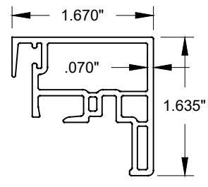
8 LOCK RAIL
