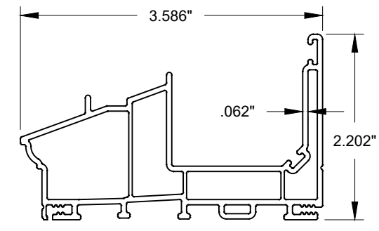
4 SILL, EQUAL LEG
