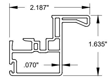
9 LIFT RAIL
