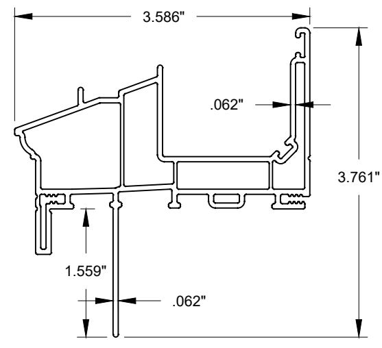
6 SILL, W/NAILING FIN
