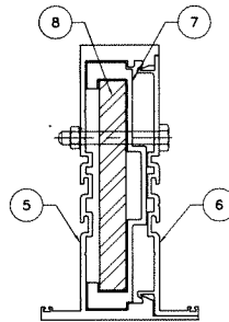
MULLION 'M3'
