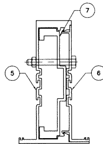
MULLION 'M2'
