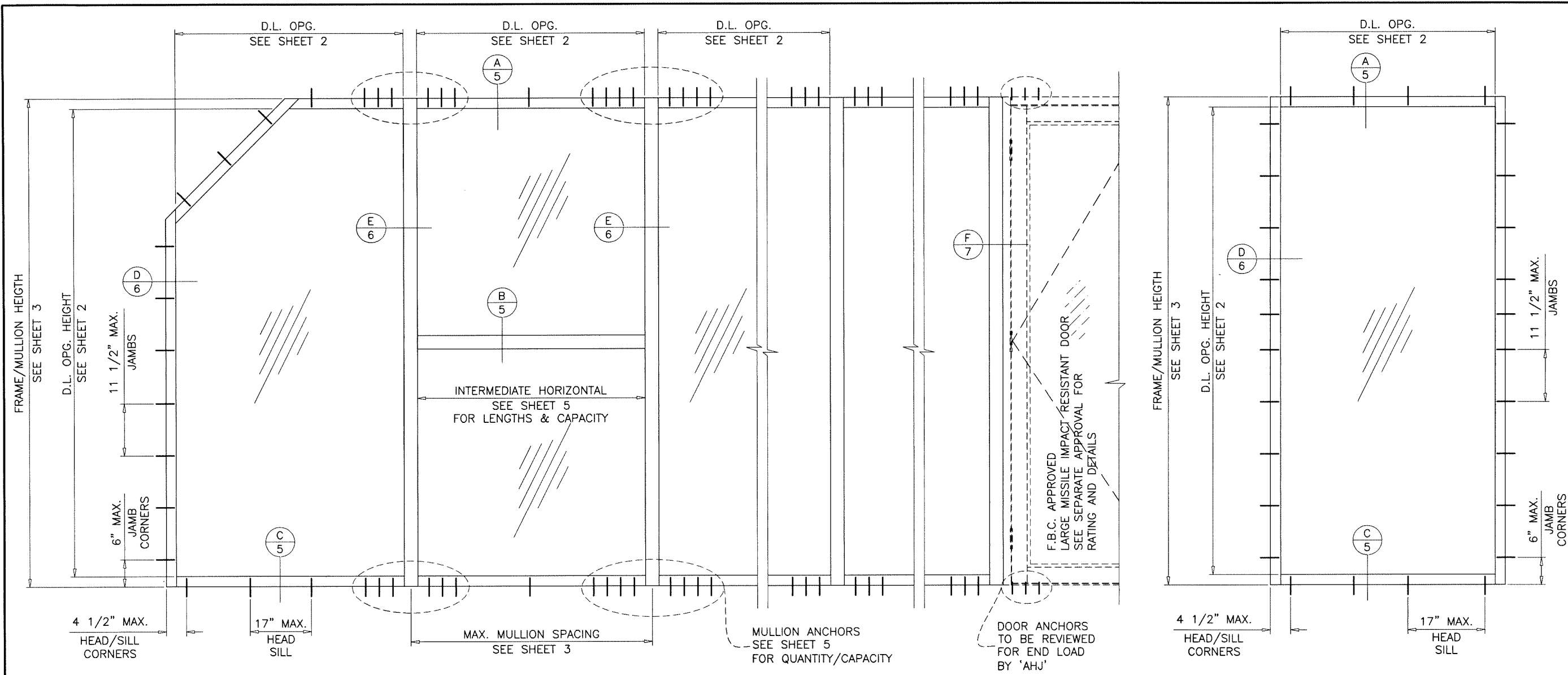
TYPICAL ELEVATIONS
