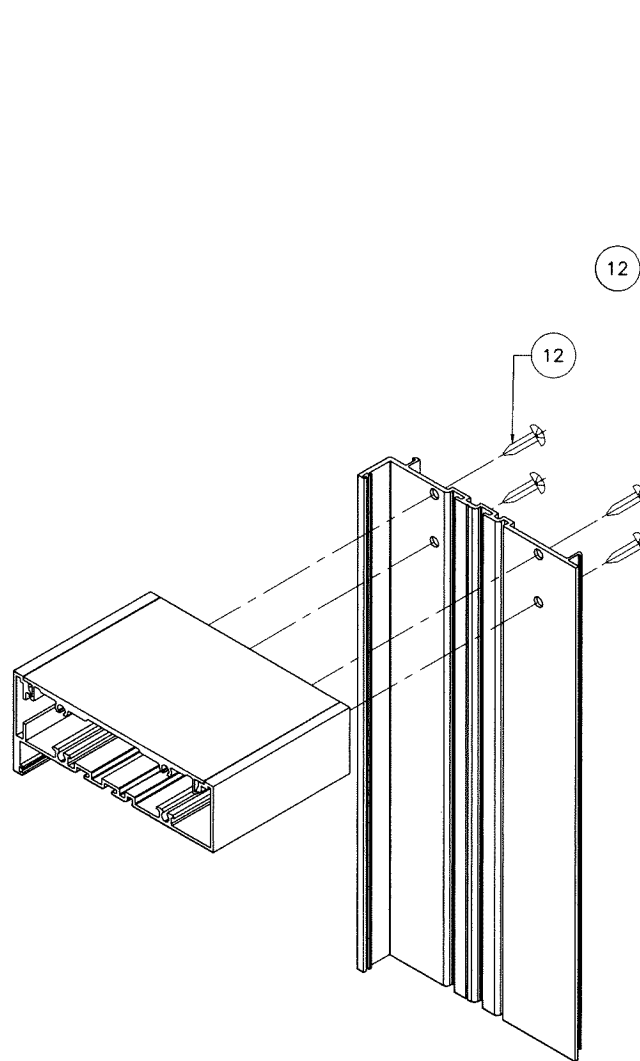
MULLION CORNER
