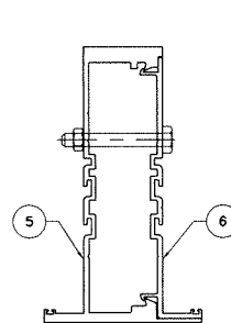
MULLION 'M1'
