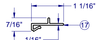
PVC SCREEN CATCH S-6226
