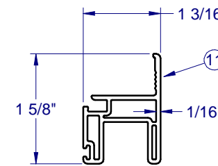
PVC SASH RAIL/STILE H-6225
