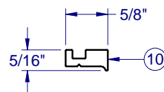
REINF. SBR/SSR S-2129
