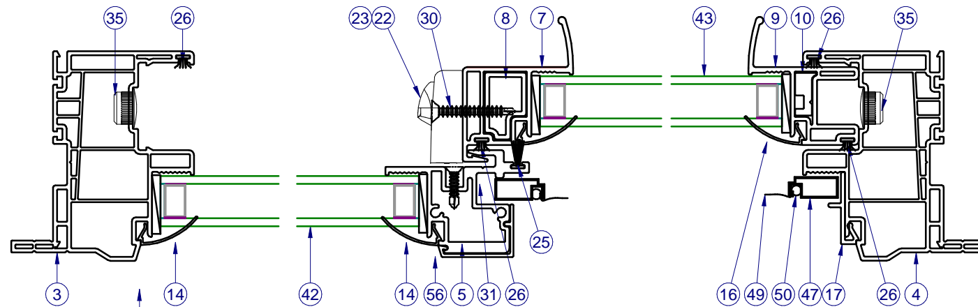
SECTION VIEW B-B
