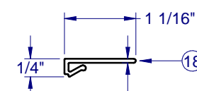
PVC SCREEN SUPPORT S-6227
