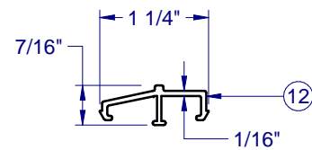
ROLLER TRACK S-1776
