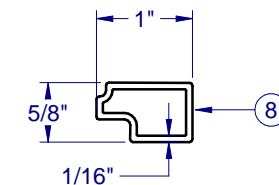
REINF. SASH MTG RAIL H-2124
