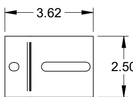
Track Clip (Opt.) .09 Galv. Steel
