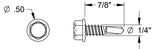
Self-Drilling Screw
