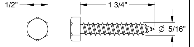
Hex Head Lag Screw
