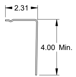
2" Angle Mount (Opt.) .086 Galv. Steel
