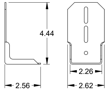
Top Fixture .085 Galv. Steel
