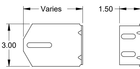
Track Bracket .116 Galv. Steel
