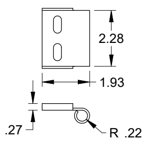
Roller Carrier .085 Galv. Steel Attached to Top Fixture w/(2) Track Bolts and Whiz Nuts
