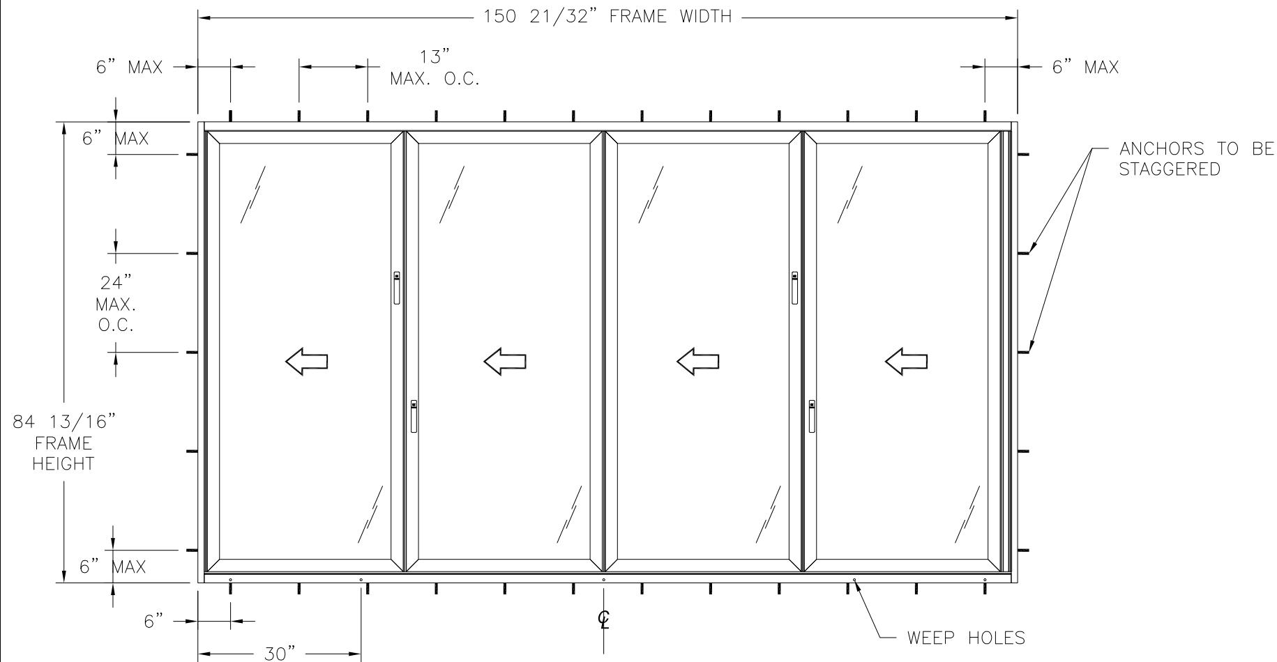
AZ57-HWF2 TWIN CORE ALUMINUM BIFOLD DOOR INTERIOR VIEW
