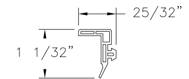
⑮ TOP TRACK GASKET RUBBER
