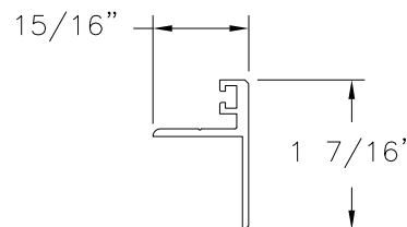
⑦ WINDOW FLANGE ALUMINUM 6063-T5
