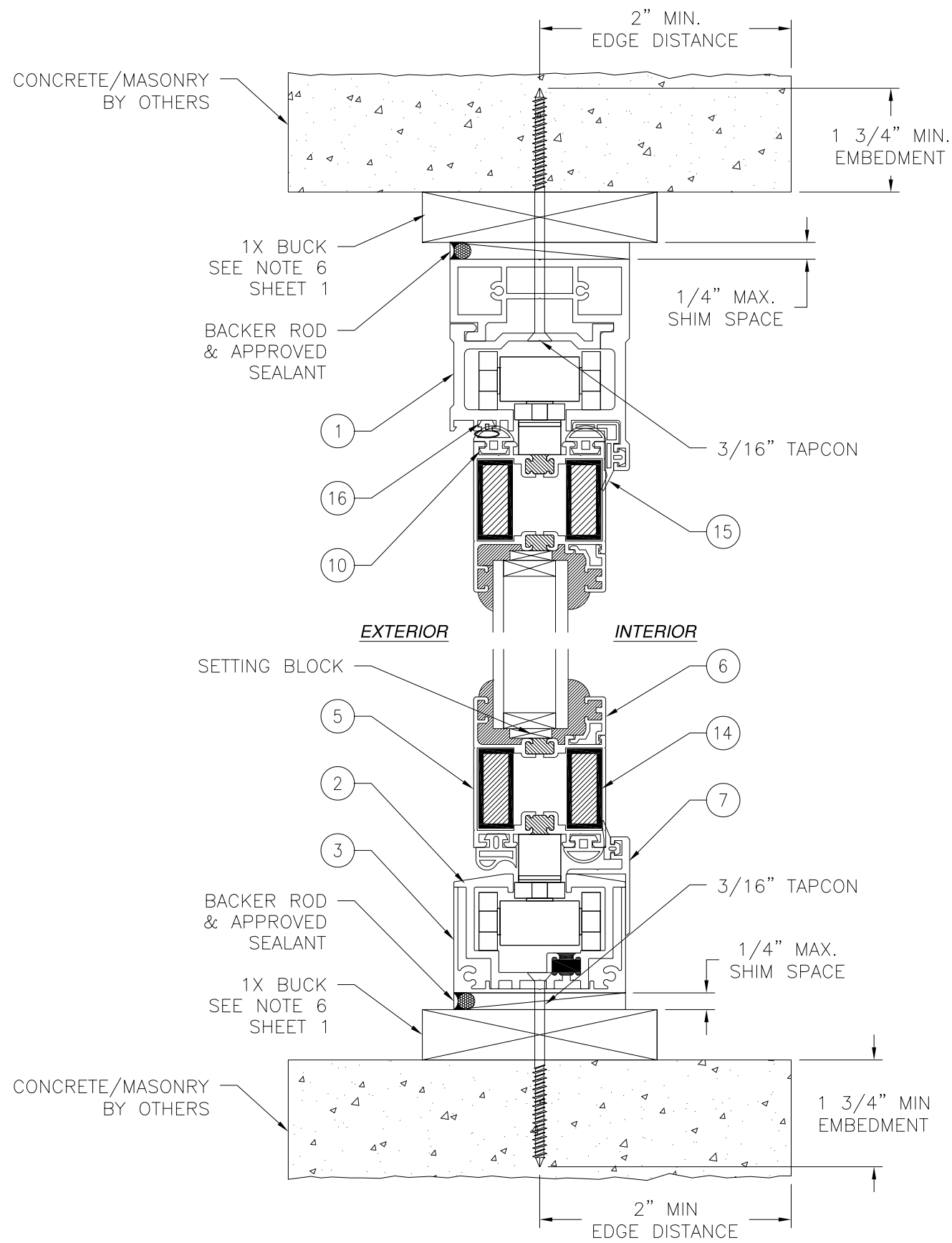
VERTICAL CROSS SECTION CONCRETE/MASONRY W/1X BUCK INSTALLATION
