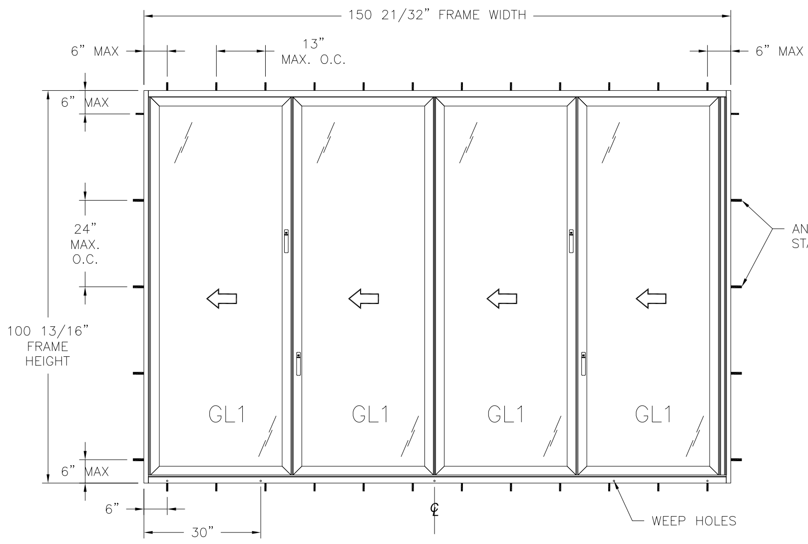
AZ57-HWF2 TWIN CORE ALUMINUM BIFOLD DOOR INTERIOR VIEW
