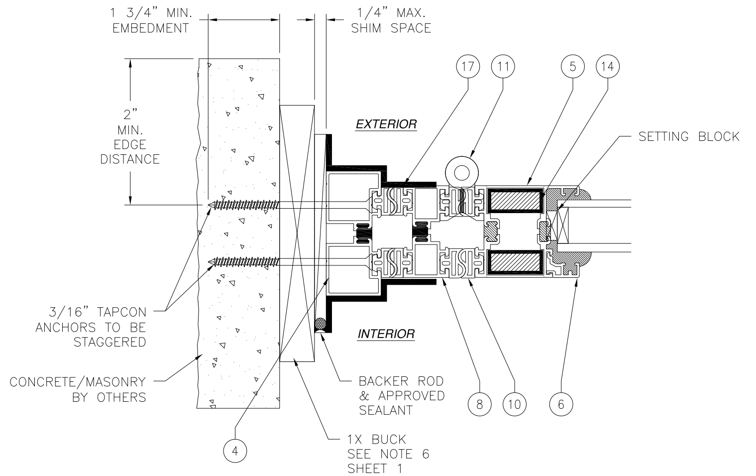
JAMB INSTALLATION DETAIL CONCRETE/MASONRY W/1X BUCK INSTALLATION
