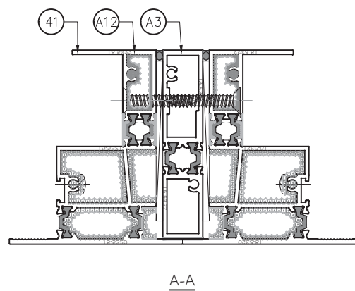
MULLION TYPE 1
