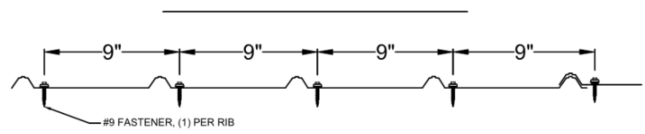
METHODS C, D, PANEL INTERIOR
