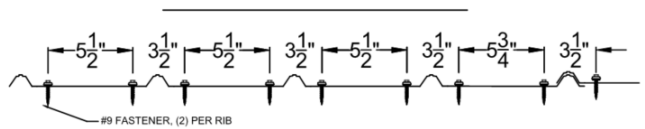
METHODS C, D, PANEL ENDS
