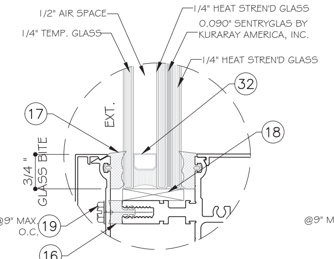
GLASS TYPE 'E' 1-5/16" NOMINAL OVERALL
