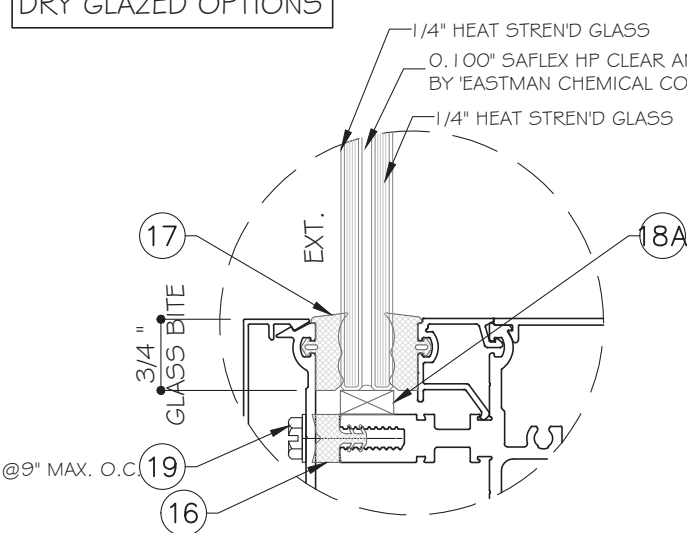
GLASS TYPE 'A' 9/16" NOMINAL OVERALL
