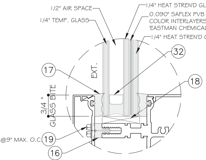
GLASS TYPE 'B1' 1-5/16" NOMINAL OVERALL
