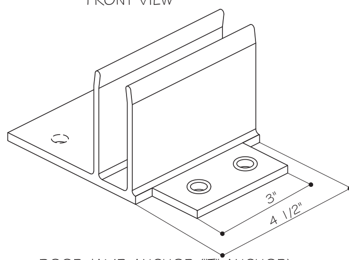
DOOR JAMB ANCHOR ("T" ANCHOR) 3D VIEW
