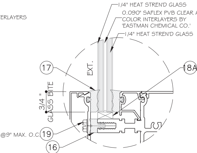
GLASS TYPE 'B' 9/16" NOMINAL OVERALL
