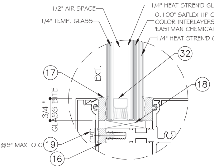
GLASS TYPE 'A1' 1-5/16" NOMINAL OVERALL
