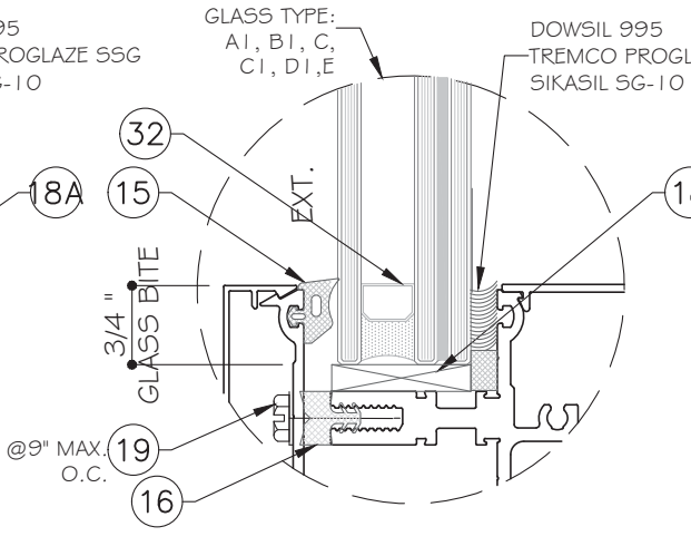
1-5/16" INSULATED LAMINATED GLASS
