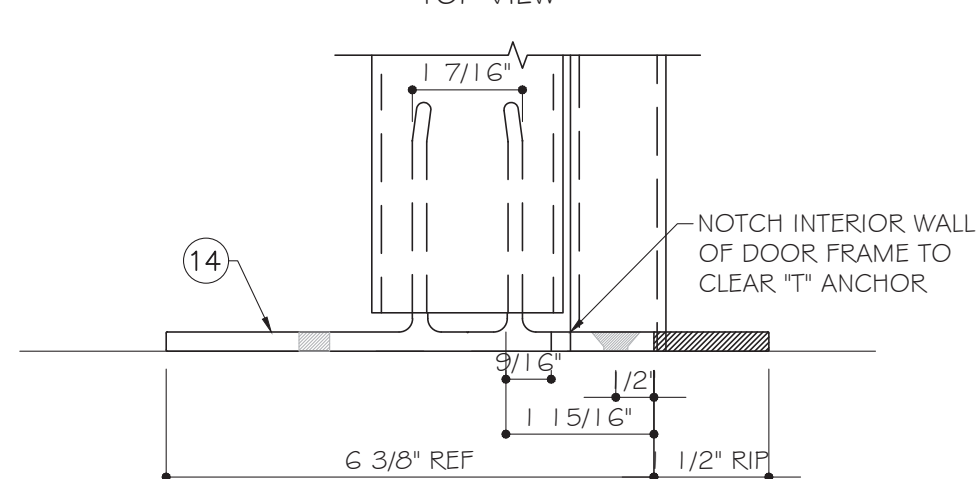
MULLION ANCHOR ("T" ANCHOR) FRONT VIEW
