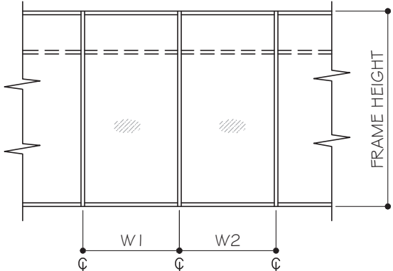
WIDTH (W) = \frac{W1 + W2}{2}
