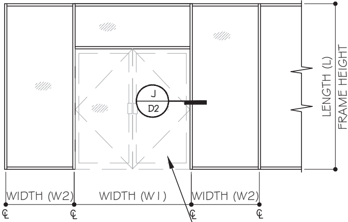
WIDTH (W) = \frac{W1 + W2}{2} REFER TO SEPARATE FLORIDA APPROVED IMPACT DOOR
