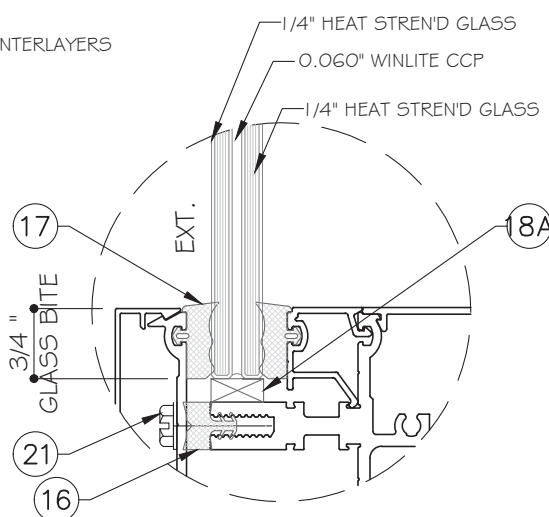
GLASS TYPE 'B' 9/16" NOMINAL OVERALL
