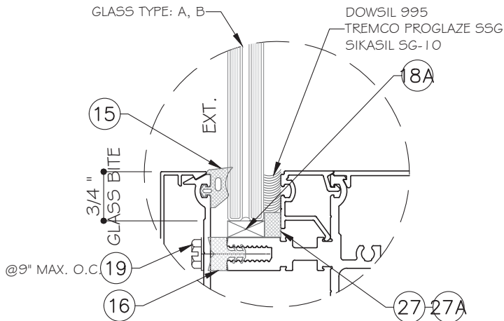
9/16" LAMINATED GLASS
