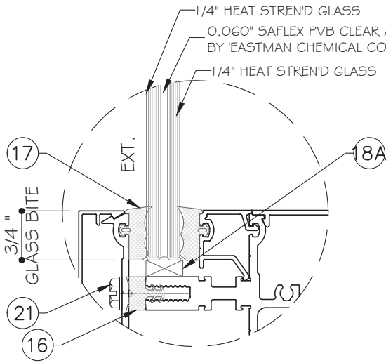
GLASS TYPE 'A' 9/16" NOMINAL OVERALL
