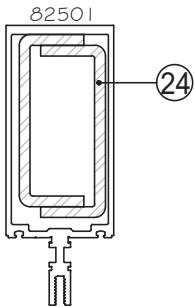
MULLION (M2)
