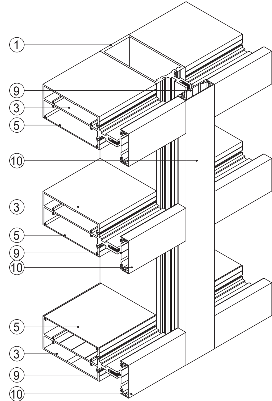
SB751 IMPACT CURTAIN WALL SYSTEM
