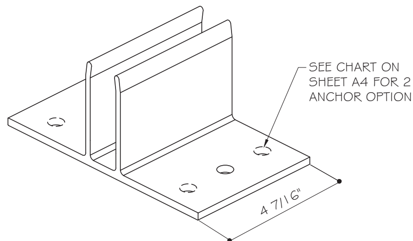
MULLION ANCHOR ("T" ANCHOR) 3D VIEW
