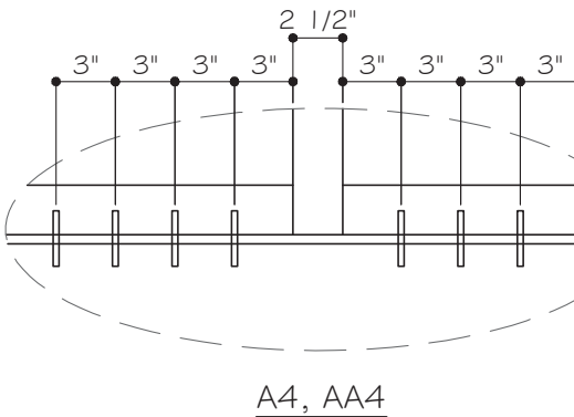
ANCHOR THRU FRAME
