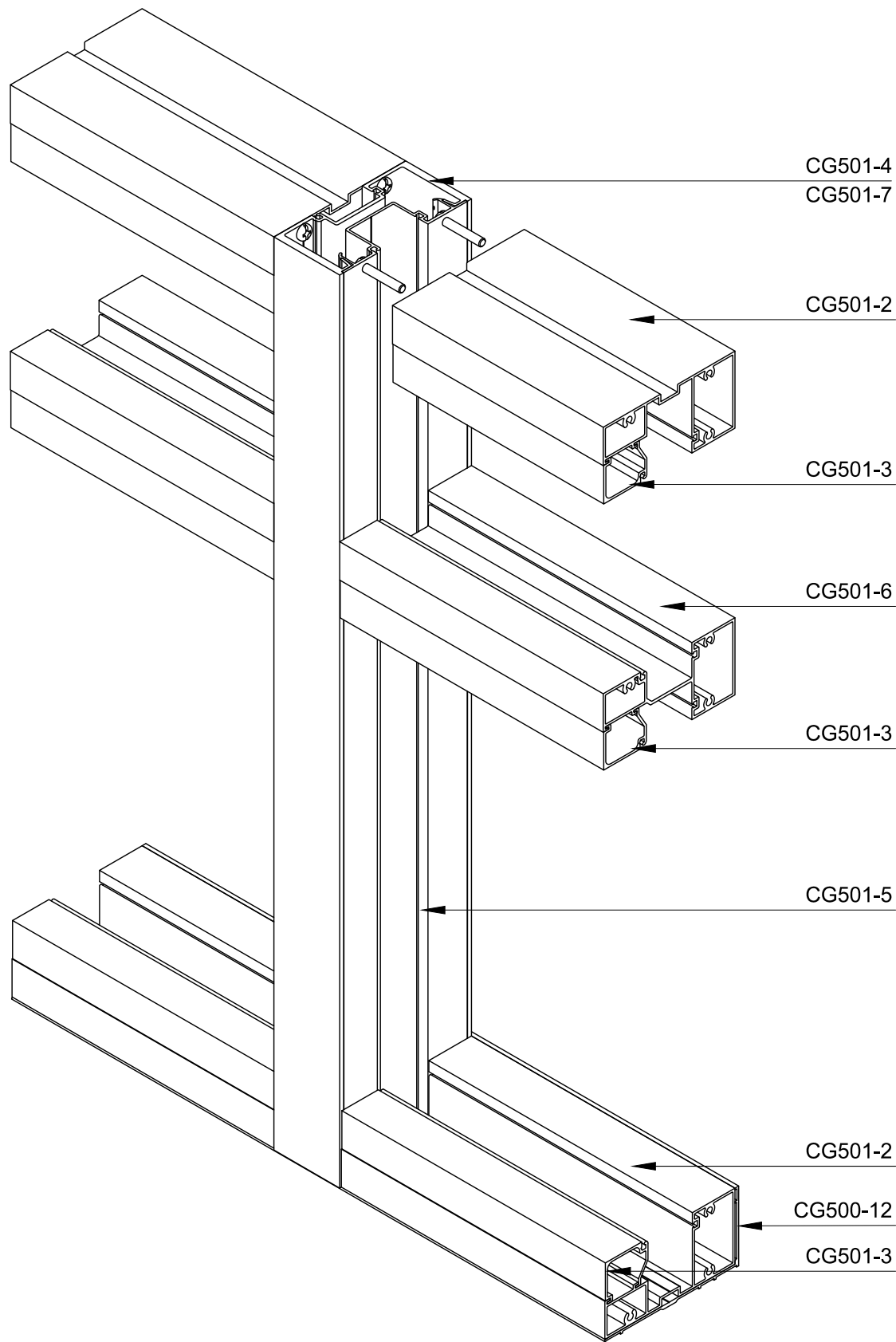
CG501 IMPACT STOREFRONT SYSTEM
