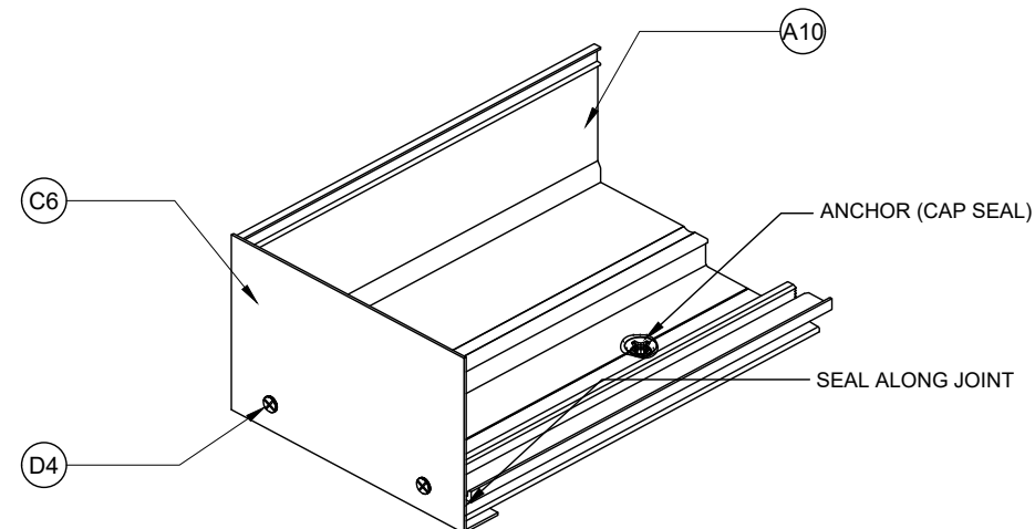
END DAM CONNECTION DETAIL AT CG501-39 STARTER SILL
