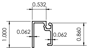
A13 TRANSOM GLASS STOP DF107
