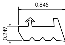
B4 INT. GASKET - DRY GLAZED RG-13
