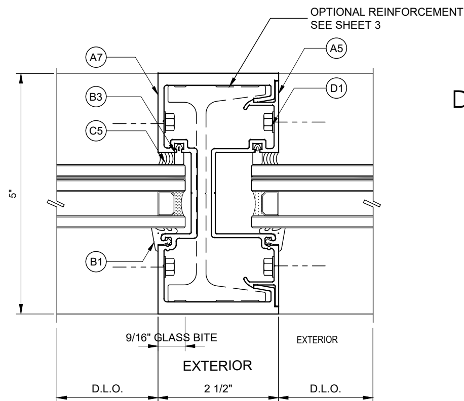
2 INTER. VERT. (MULLION)
