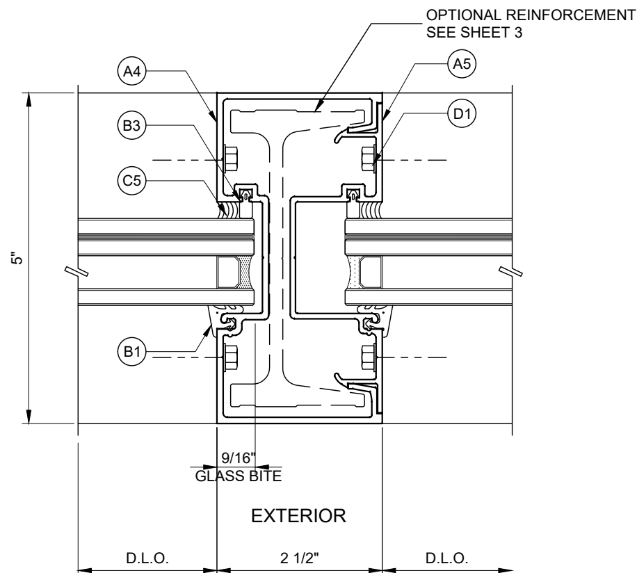
1 INTER. VERT. (MULLION)
