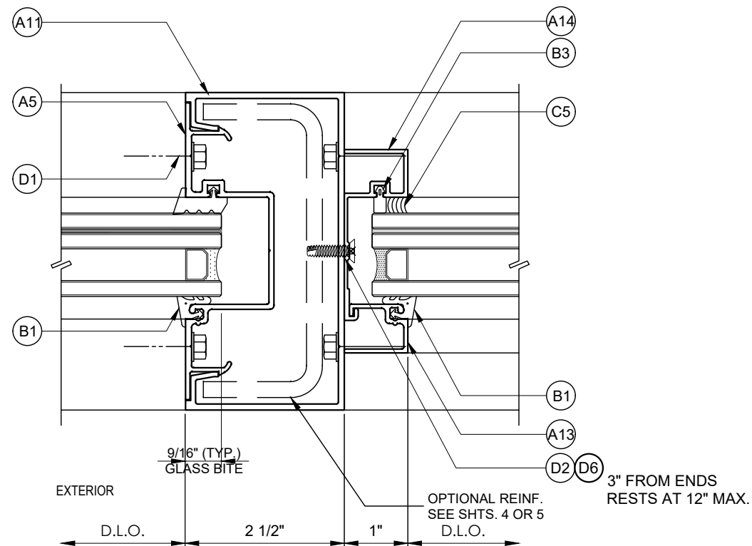
2 TRANSOM DOOR JAMB AT SIDELITE
