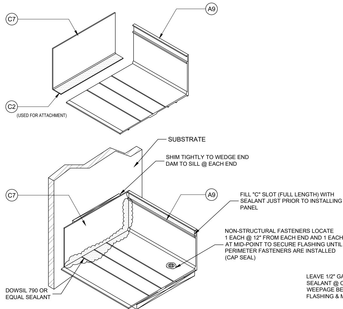
END DAM CONNECTION DETAIL AT CG500-12 STARTER SILL
