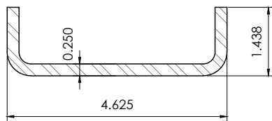
C9 STEEL REINF. (A572, GR. 50) ST500-4
