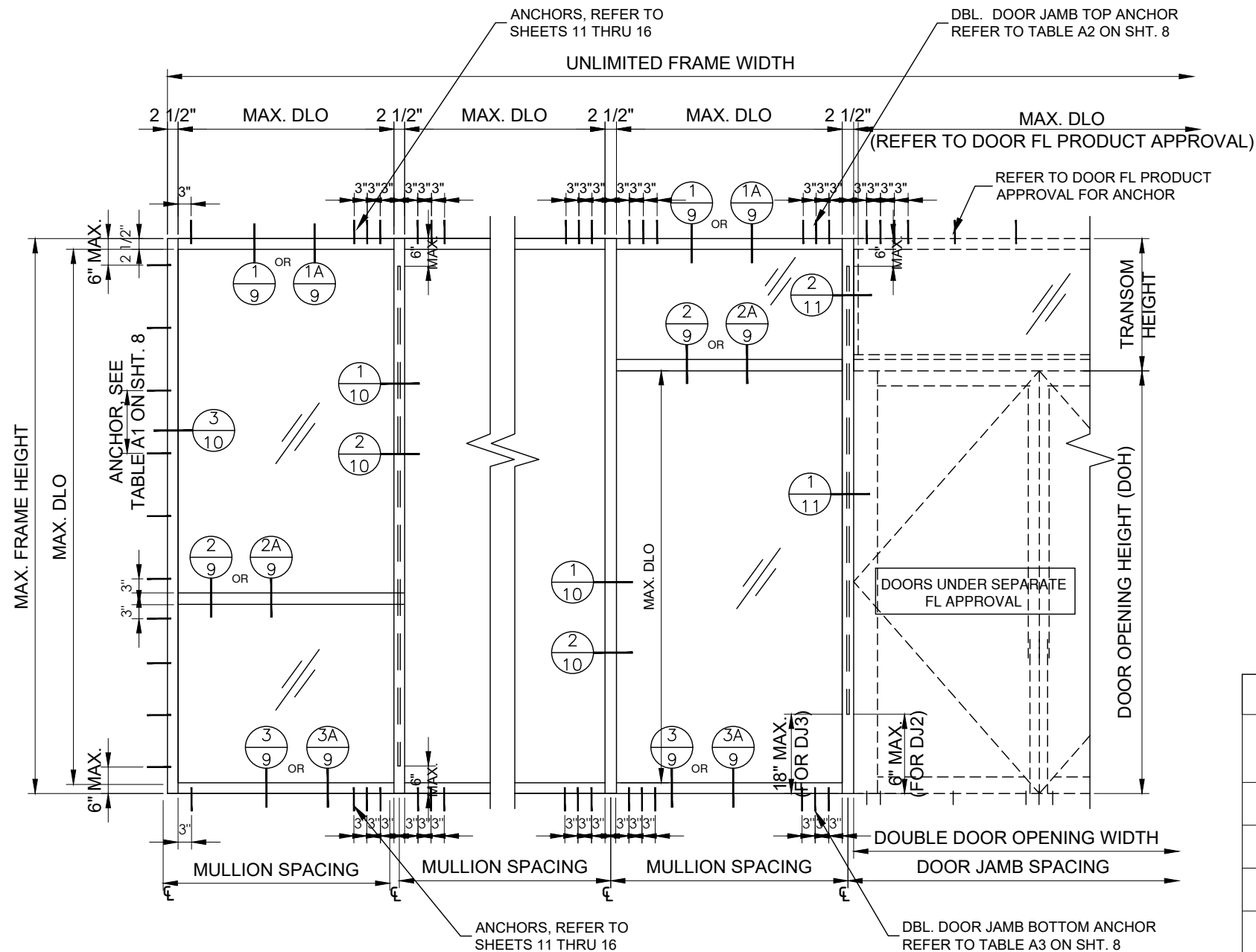
TYPICAL ELEVATION
