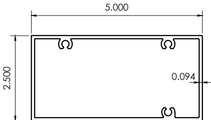
A15 DOOR TRANSOM DF500-2
