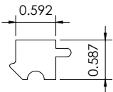
B6 SETTING BLOCK AT INV. HOR. RSB-12
