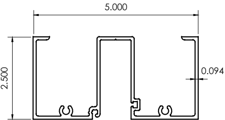
A1 JAMB / HEAD CG500-11
