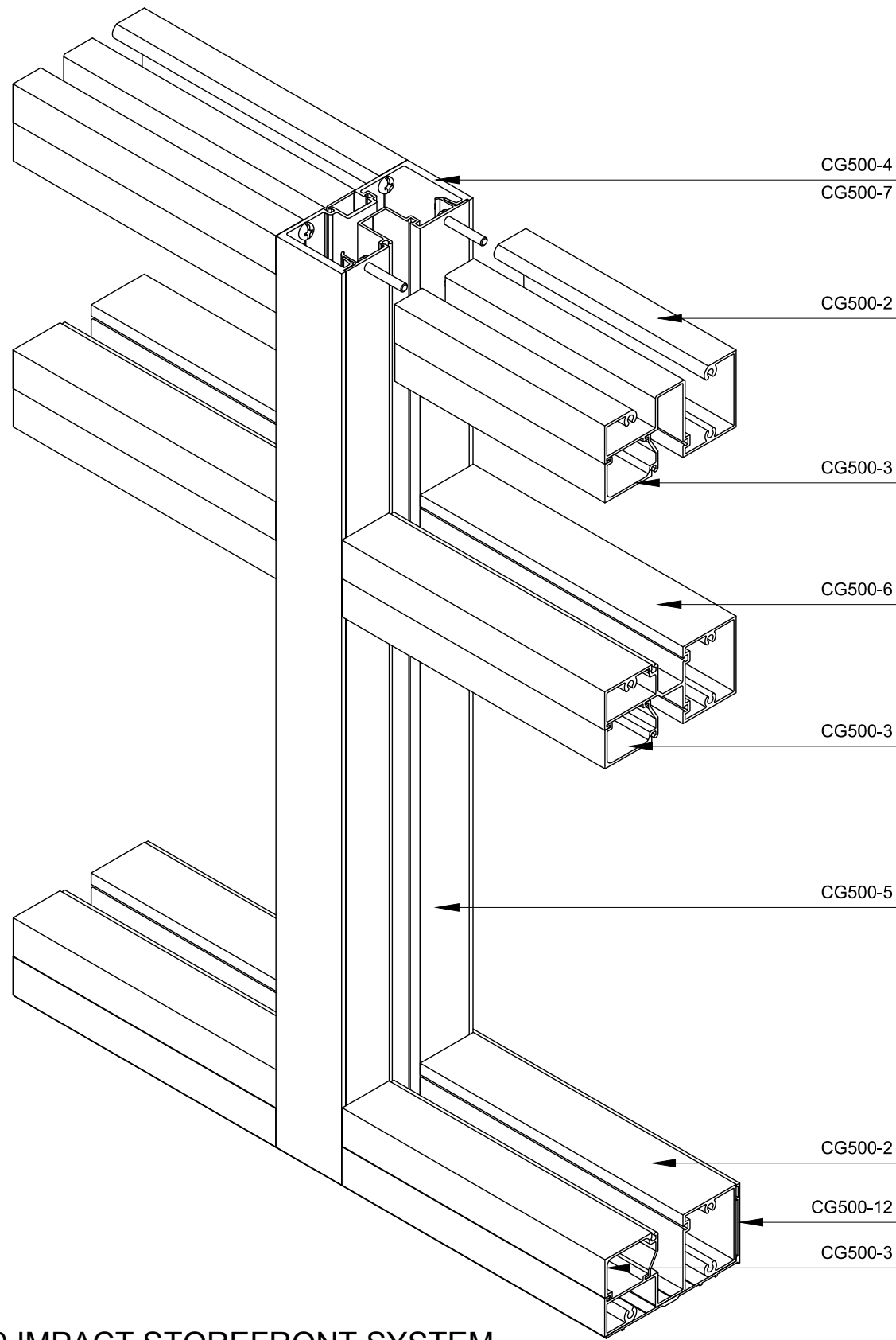
CG500 IMPACT STOREFRONT SYSTEM
