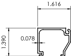
A3 GLASS STOP CG500-3
