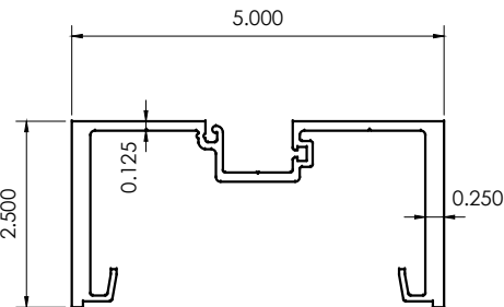
A7 HVY. VERTICAL MULLION CG500-7
