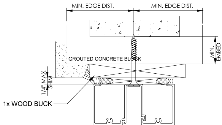
TYPE E or EE
