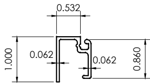
A13 9/16" GLASS STOP DF107
