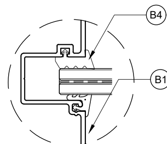
DRY GLAZE DETAIL (OPTION)
