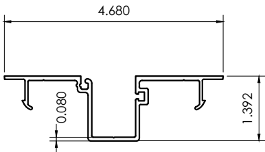
A5 OPEN BACK MULLION FILLER CG500-5
