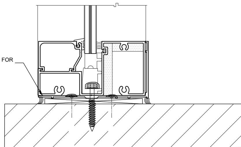
DETAIL "A-A"
