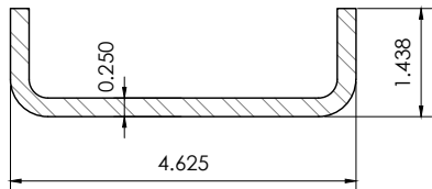
C9 STEEL REINF. (A572, GR. 50) ST500-4
