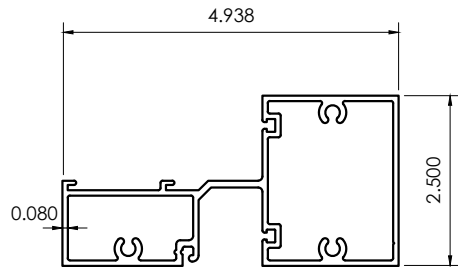
A6 INTERMEDIATE HOR. CG500-6
