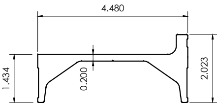
A8 ALUMINUM REINFORCEMENT DF500-4
