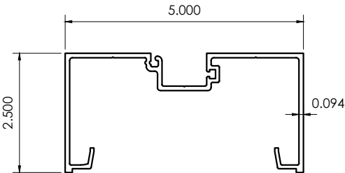
A4 LIGHT VERTICAL MULLION CG500-4
