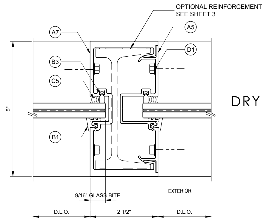
2 INTER. VERT. (MULLION)
