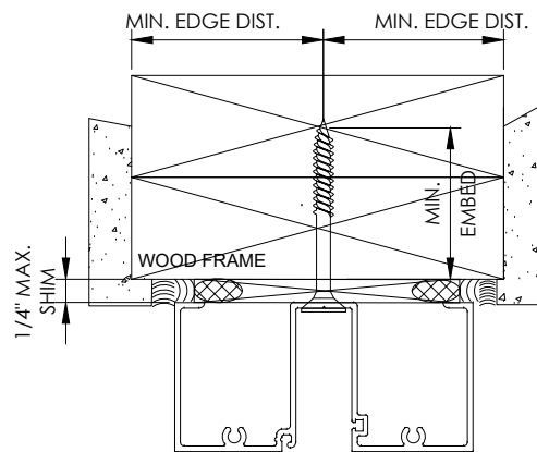
TYPE A, AA, B or BB
