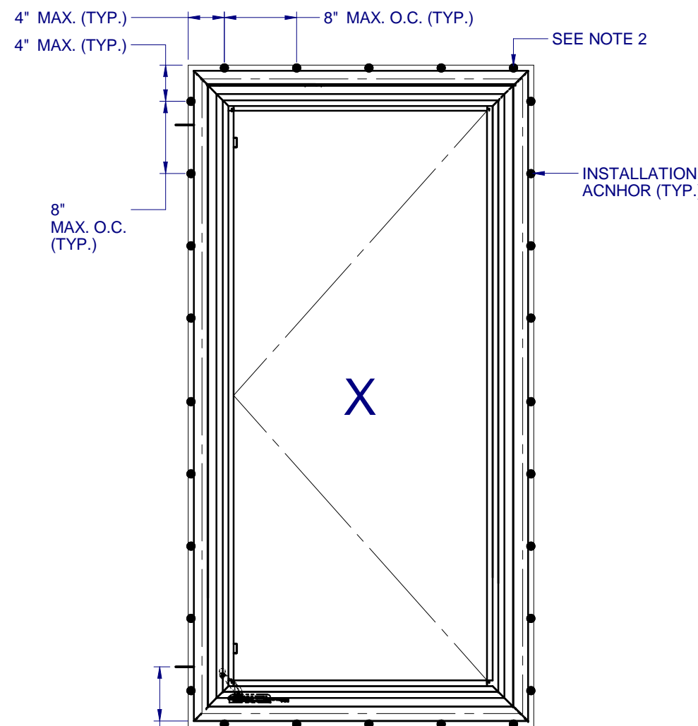
ANCHOR LAYOUT - (FIN)
