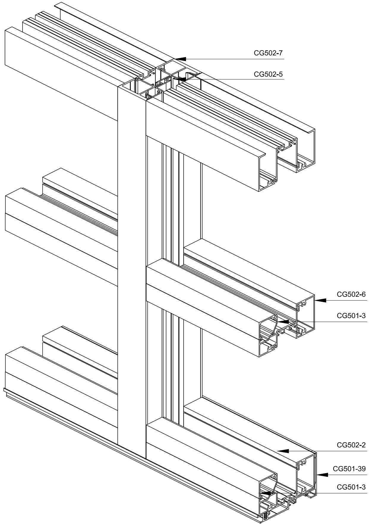
CG502 IMPACT STOREFRONT SYSTEM
