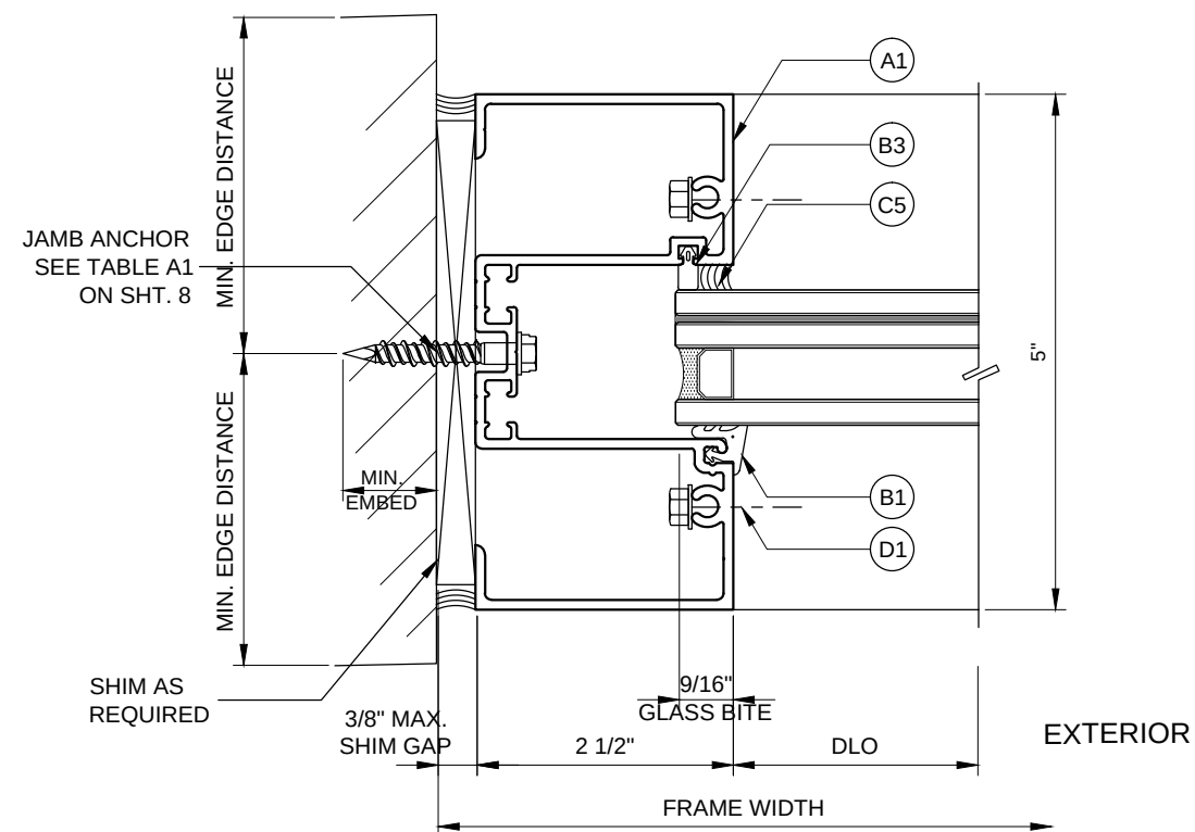
2 JAMB (ANCHORED) APPLICABLE TO MAX. PRESSURE, MAX. FRAME HEIGHT OR MAX. MULLION SPACING
