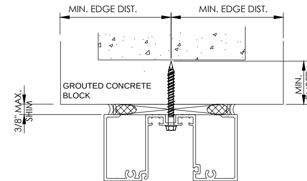
TYPES E, EE
