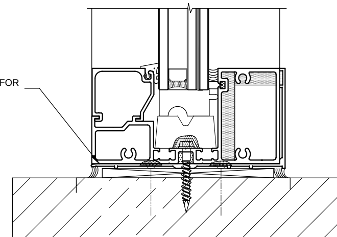
DETAIL "A-A"
