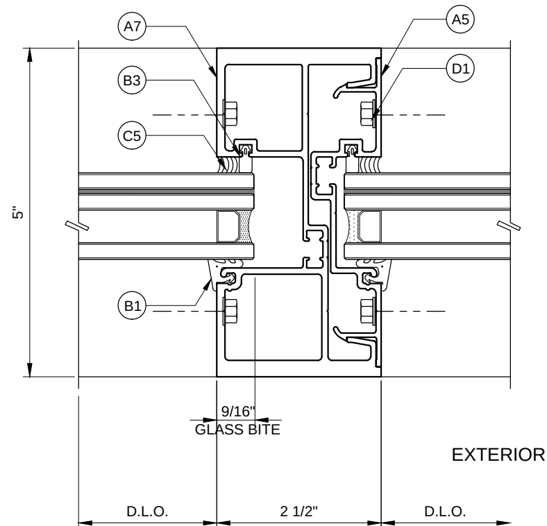
1 INTER. VERT. (MULLION)
