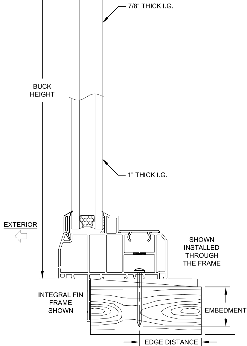
VERTICAL SECTION D-D
