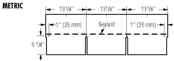
Figure 11-3: Use four nails for every full shingle.
