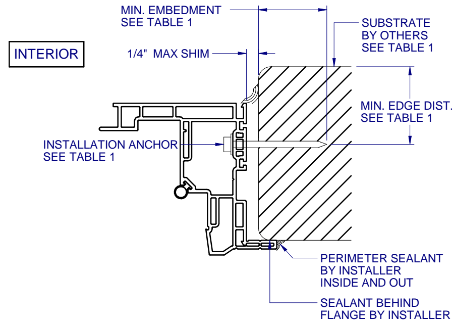
B HORIZONTAL SECTION 6 TYPICAL JAMB ANCHORAGE
