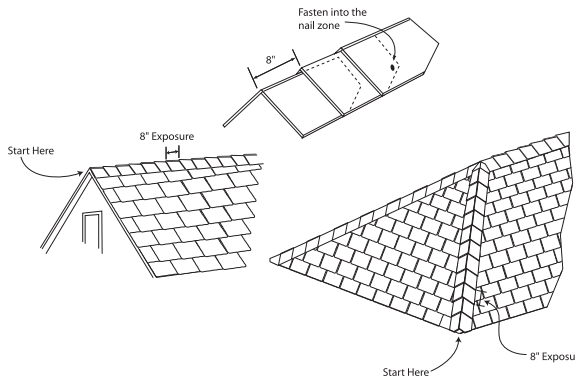
Diagram: C LAMARITE Site Made Hip & Ridge
