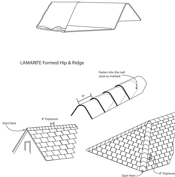
Diagram: B LAMARITE Formed Hip & Ridge
