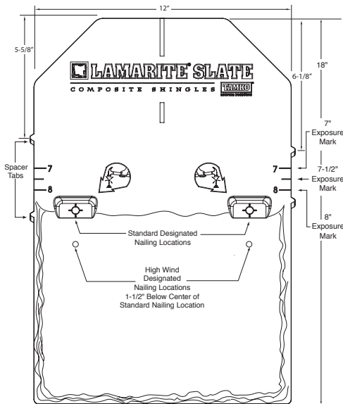
Shingle Design A
