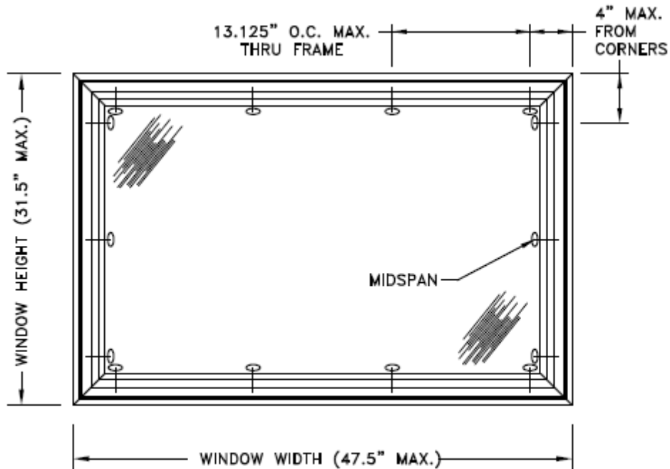
TYPICAL ELEVATION WITH FASTENER SPACING
