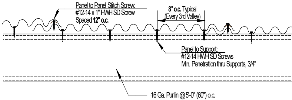
Assembly Profile View - Typical Fastening Pattern Across Row
