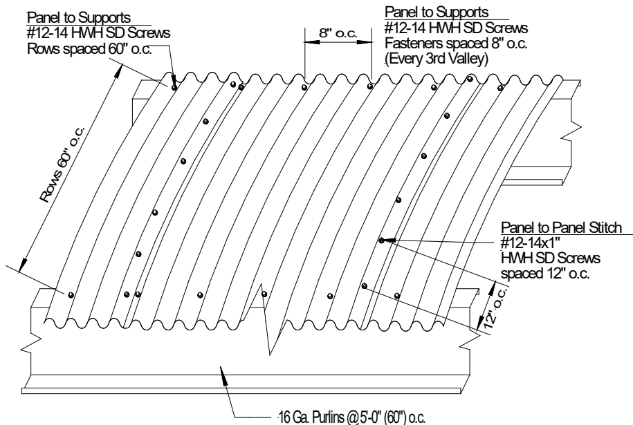
METHOD 1: Typical "Curved S-Deck" Roof Assembly Isometric View
