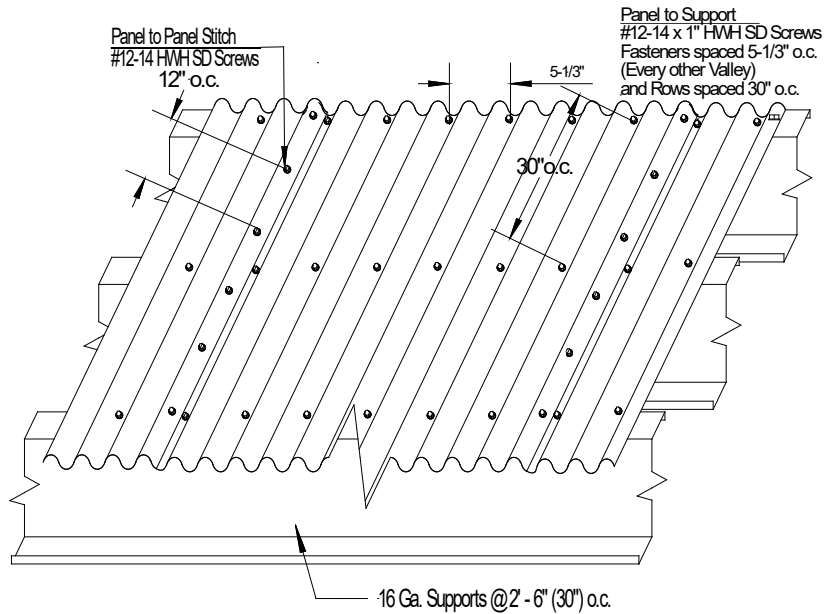
METHOD 2: Typical "S-Deck" Roof Assembly Isometric View
