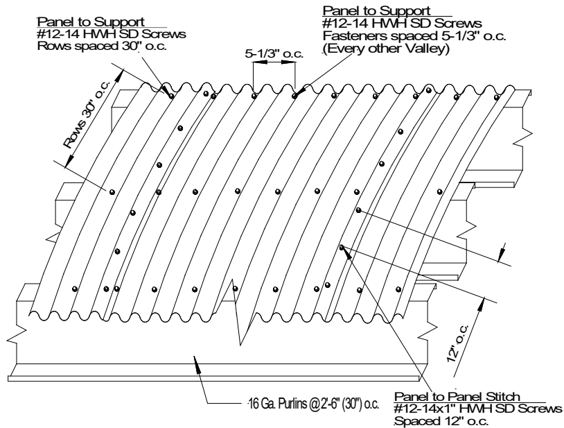
METHOD 2: Typical "Curved S-Deck" Roof Assembly Isometric View
