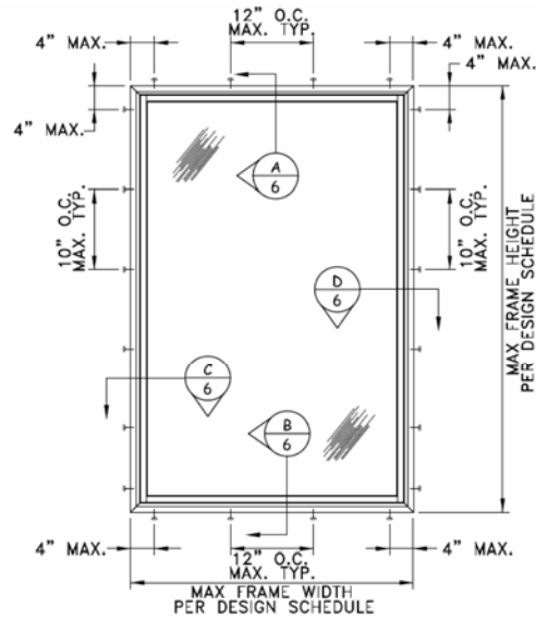
2 2 N.T.S. ANCHOR ELEVATION FOR INSTALLATION THROUGH FRAME EXTERIOR ELEV
