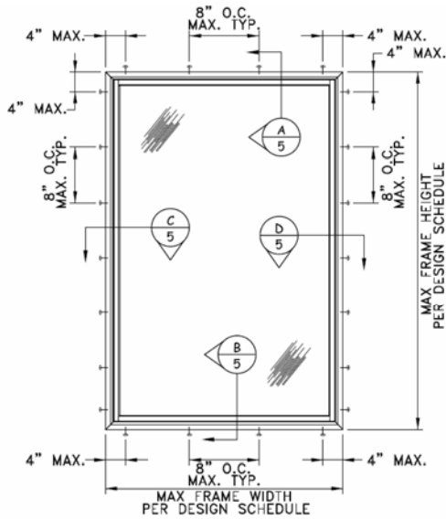
1 2 N.T.S. ANCHOR ELEVATION FOR INSTALLATION WITH NAIL FIN EXTERIOR ELEV
