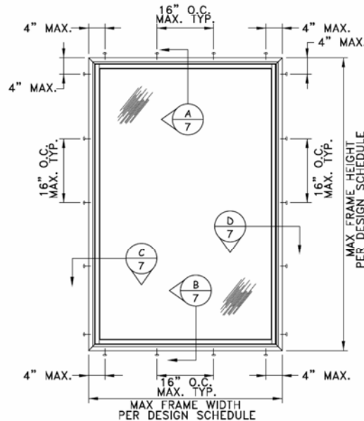
3 2 N.T.S. ANCHOR ELEVATION FOR INSTALLATION WITH STRAP EXTERIOR ELEV
