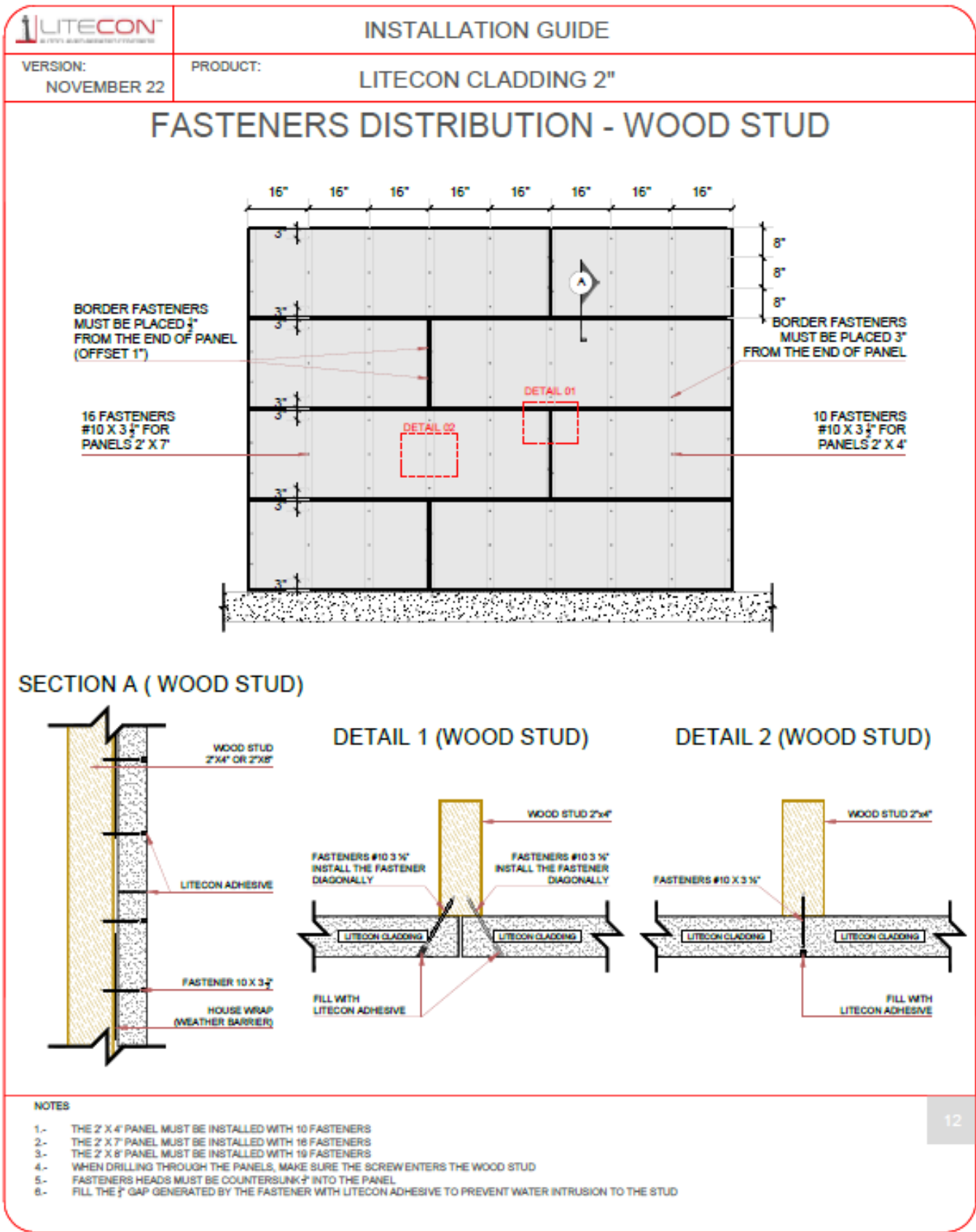
FIGURE 3- FASTENING DETAILS FOR LIGHT-FRAMED ASSEMBLIES AT MAXIMUM STUD SPACING OF 16 INCHES ON CENTER
